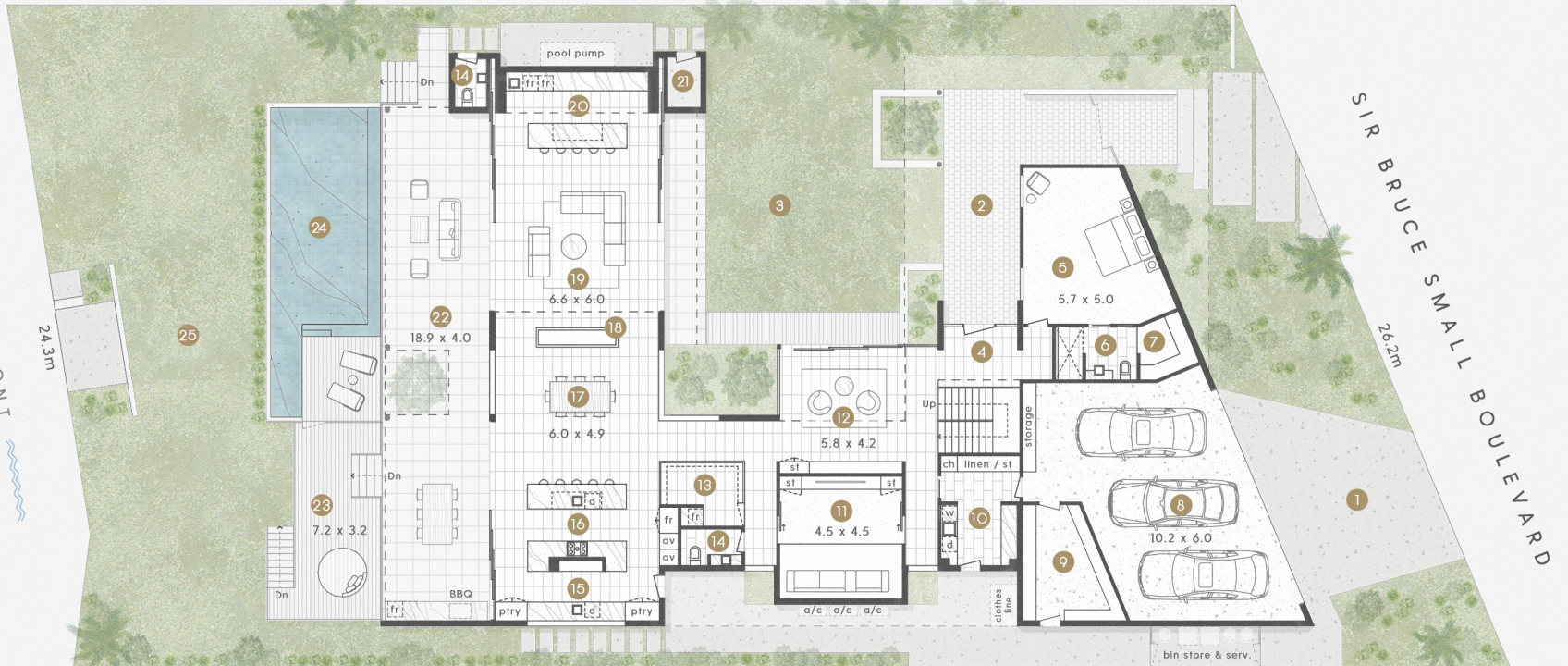
:: FLOORPLAN & SITEPLAN Ground Floor - 3.0m Ceiling
